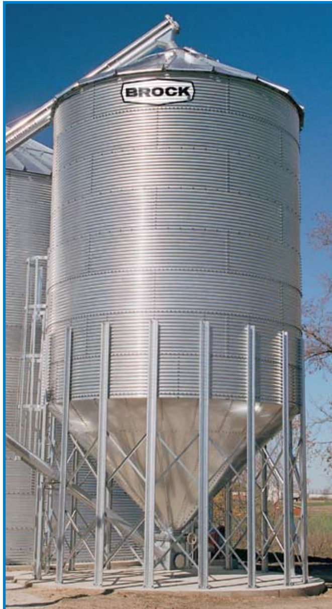
Sturdy "X" bracing between legs gives additional bin strength. Bracing is simple to assemble and offers access to boot.
