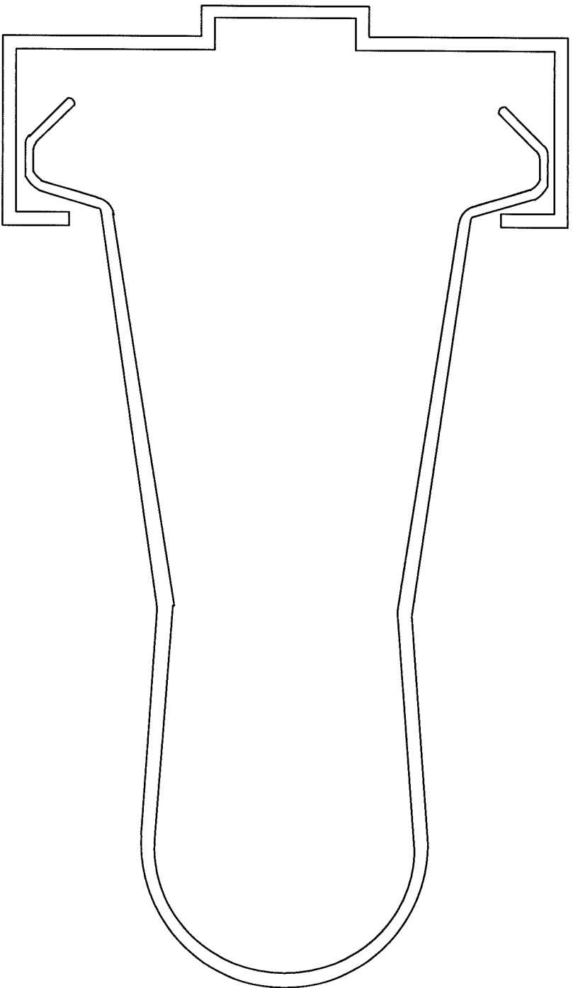
Wire Masonry Anchor (new wall)
