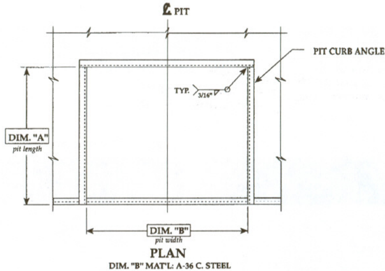
FIGURE B – PLAN VIEW
