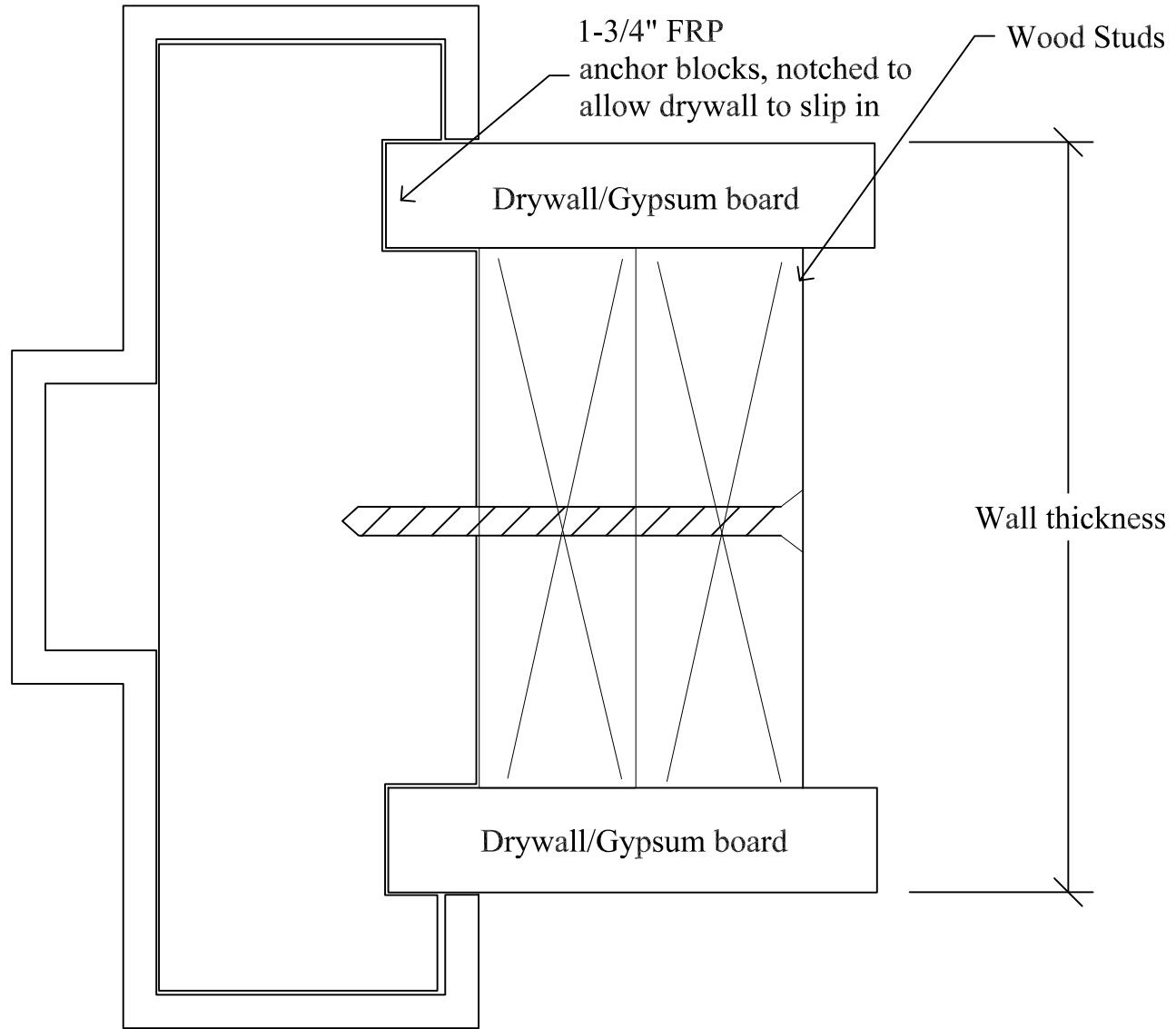
Wood Stud Anchor (new wall)
